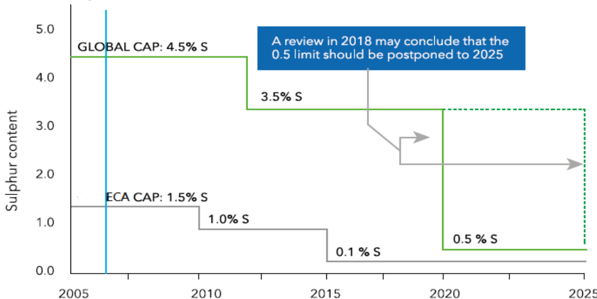
Figure 1. MARPOL Annex VI fuel sulphur content limits
